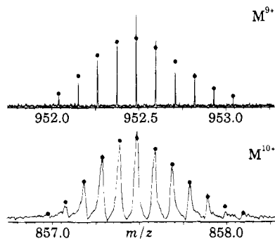
Figure 5. Partial ESI/FT mass spectrum of ubiquitin ions (top) trapped during a 10^{-4} -s spraying 20 \mu\text{M} at 150 \text{ mL/min} ( 5 \times 10^{-18} mol) and (bottom) formed by the separate introduction of 5 \times 10^{-14} mol of sample. Superimposed dots are the predicted isotopic abundances.
