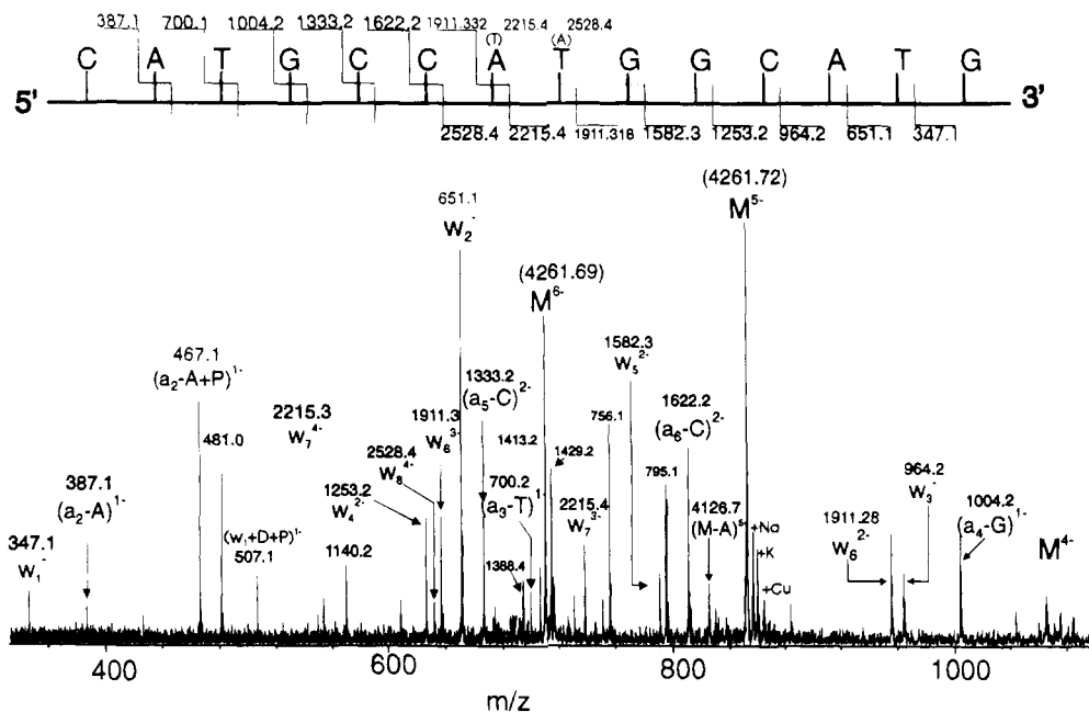
Figure 10. Negative ion ESI/FT mass spectra of a 14-mer oligonucleotide NcOI, predicted MW = 4261.75; a and w cleavages contain the 5' and 3'-termini, respectively.
